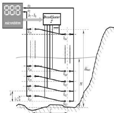
Fig.1 Scheme mounting sensors
