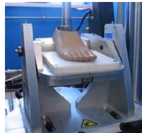
Test subassembly "ankle-foot prosthesis lower limb external"
