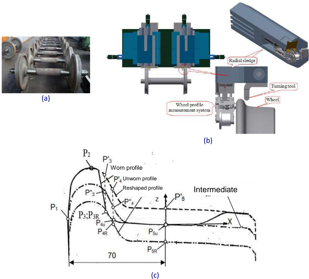
Figure 1.a. Wheelsets; b. Profile measurement system; c. Measurement points
